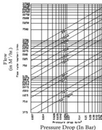
Typical pressure drop characteristics for basket with \Phi 3 mm. proportion.
